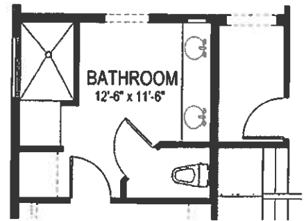
Optional Walk-in Shower Master Bath
